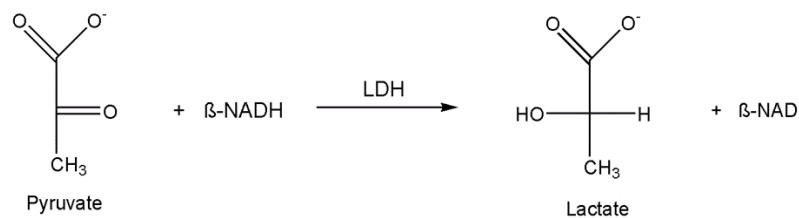
Fig 3.3 Enzymatic reaction of lactate dehydrogenase
