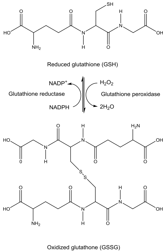
Fig.2.4 Illustration of glutathione recycling
